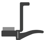
FTUS08-75 8mm Underside Tape Windshield Molding
